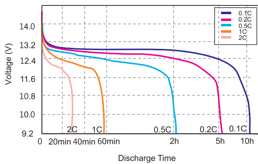
Different Rate Discharge Curve @25°C
